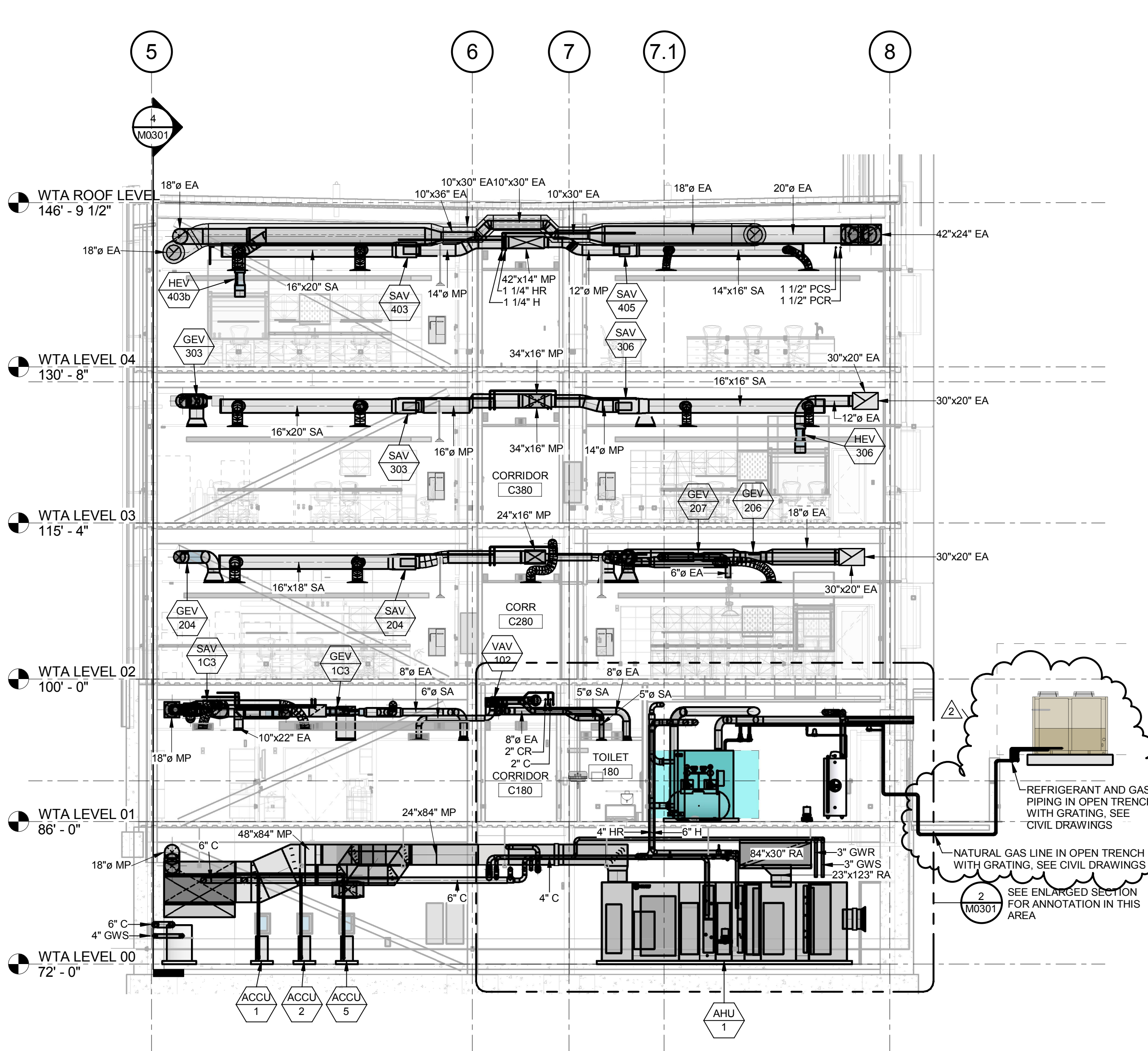
1 AREA A SECTION - (LOOKING NORTH) 1/8" = 1'-0"
