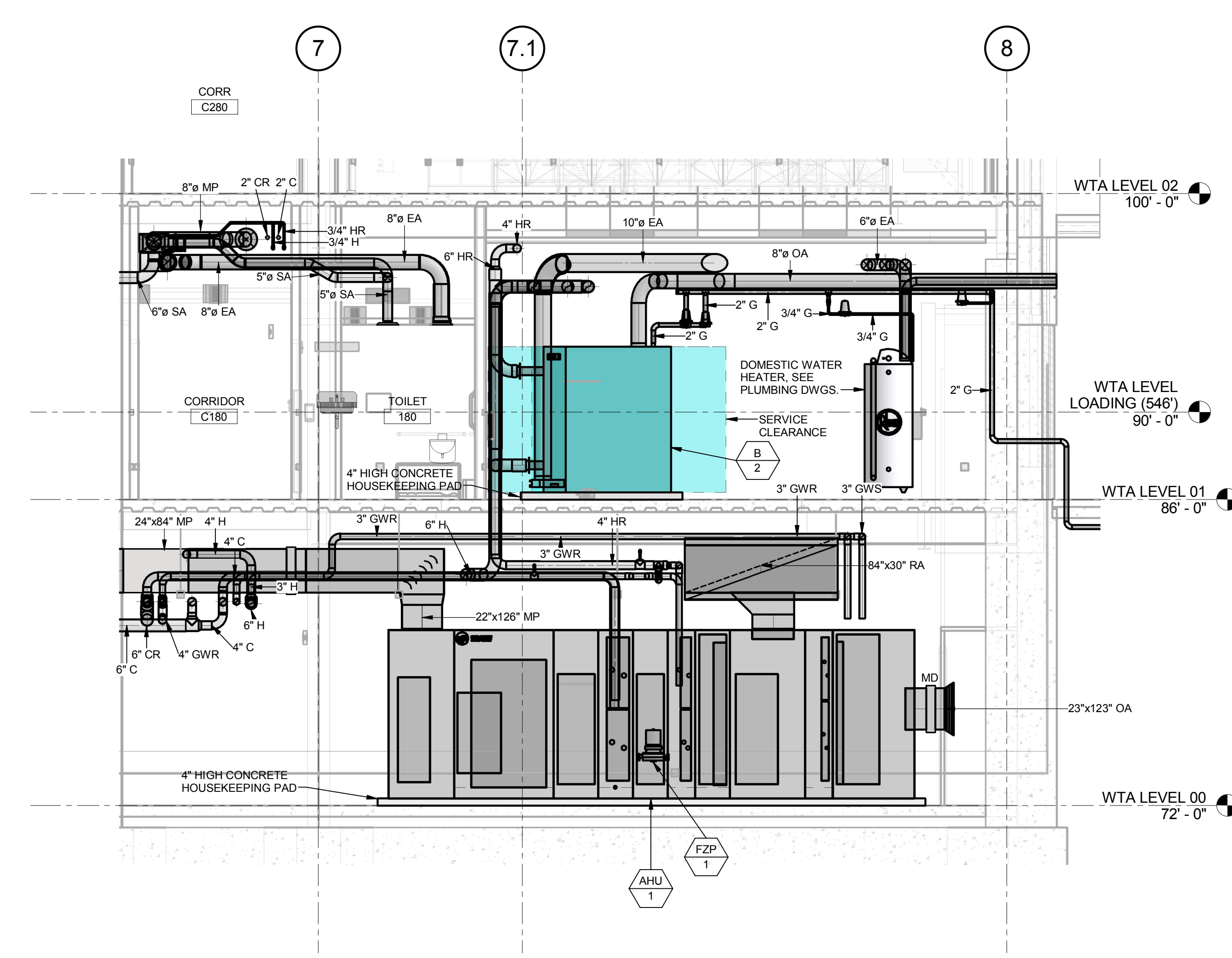
2 EAST WING SECTION (NORTH) - AHU-1 1/4" = 1'-0"
